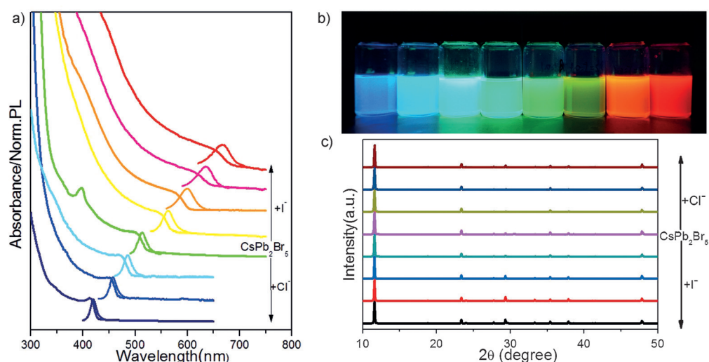
Figure 4. a) Evolution of the optical absorption (left) and PL (right) spectra of \text{CsPb}_2\text{Br}_5 nanoplatelets with increasing quantities of anion-exchange of \text{I}^- and \text{Cl}^- , respectively. b) Photograph of \text{CsPb}_2\text{Br}_5 nanoplatelets under the irradiation of a 365 nm UV lamp. c) PXRD patterns of the parent \text{CsPb}_2\text{Br}_5 nanoplatelet and anion-exchanged samples.
